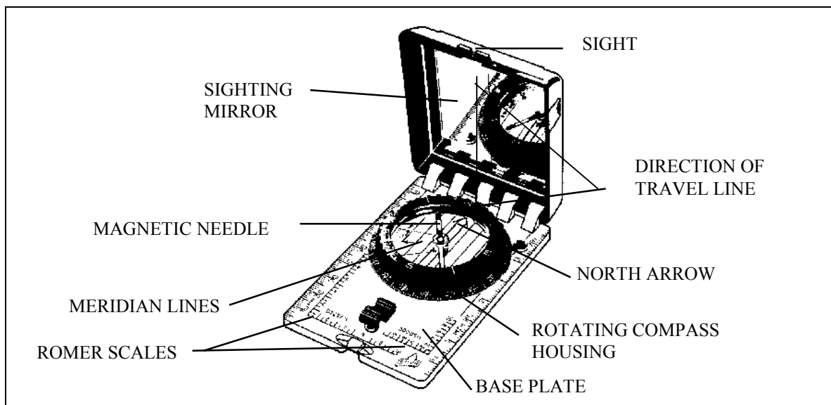
Figure 27 - The "SILVA" orienteering compass [Type 15T]
